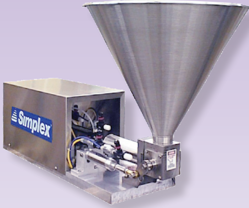
Simplex Model AAS-100 Table-Top with straight spout, product cylinder and 20 gallon hopper
