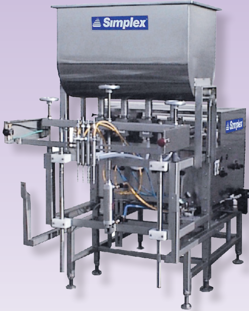
Automated Simplex Model AAS-400 Four-head with plunging head plug spouts and 20 gallon "U" shaped hopper
